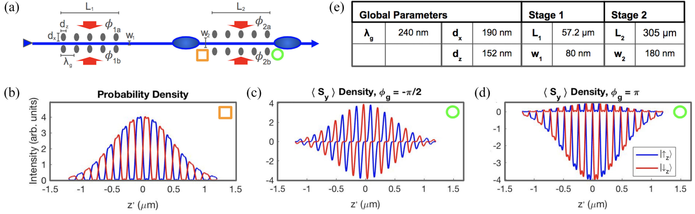
FIG. 2. Spin-dependent electron densities. (a) Experimental schematic. The positions where the electron density or spin density is calculated are highlighted by an orange square and a green circle. (b) Spin-dependent electron probability density distribution after interaction with first stage and free-space drift; input spin states differentiated by color. (c),(d) Electron y-axis spin density immediately following interaction with the second stage: (c) has a relative interaction phase between stage 1 and 2 of -\pi/2 , leading to \langle S_y \rangle \approx 0 ; (d) has a relative interaction phase between stage 1 and 2 of \pi , which results in \langle S_y \rangle \approx -0.7\hbar/2 . (e) Summary of example pillar geometry values as denoted in (a).
