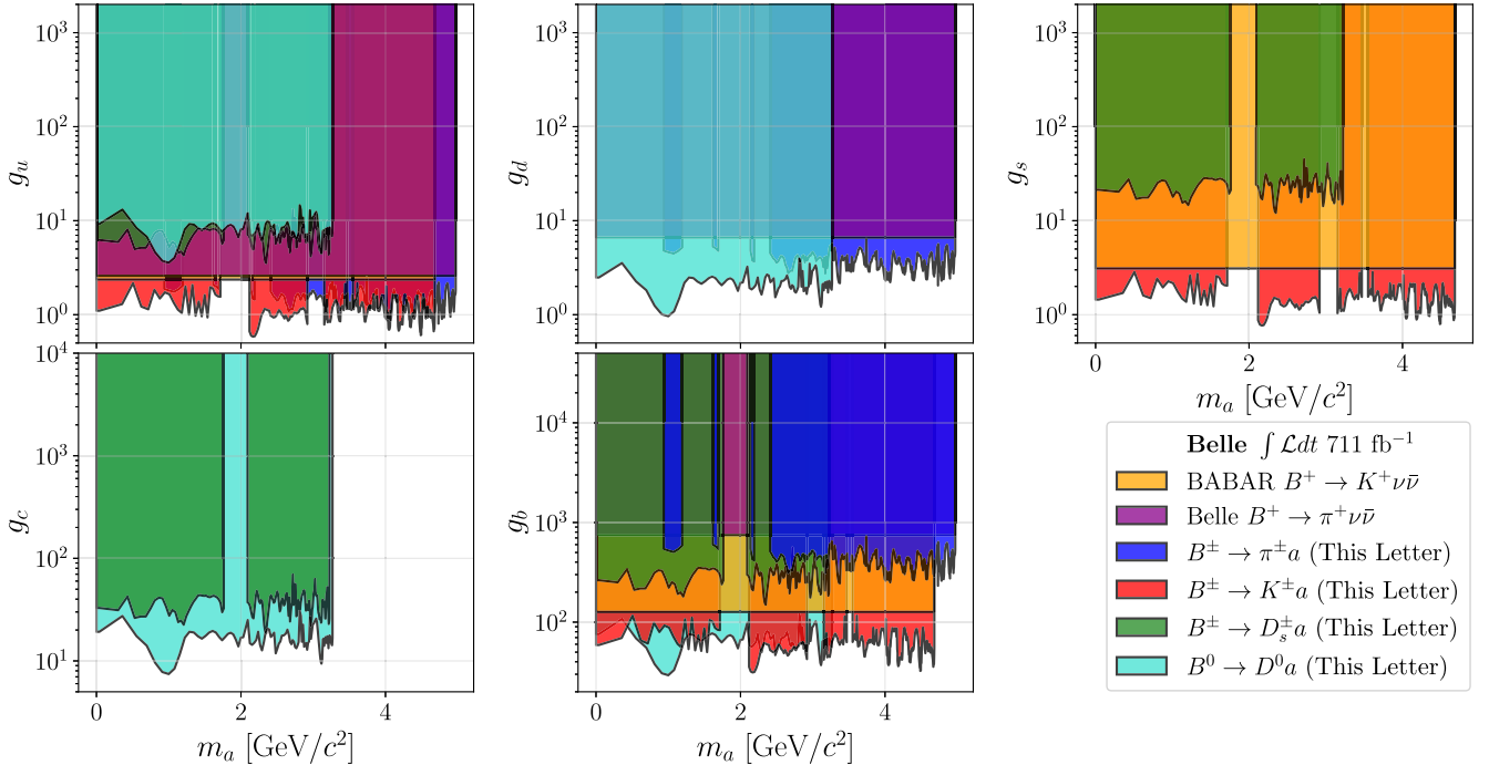
FIG. 5. 90% confidence level exclusion regions on the ALP-quark couplings described in Ref. [19].
