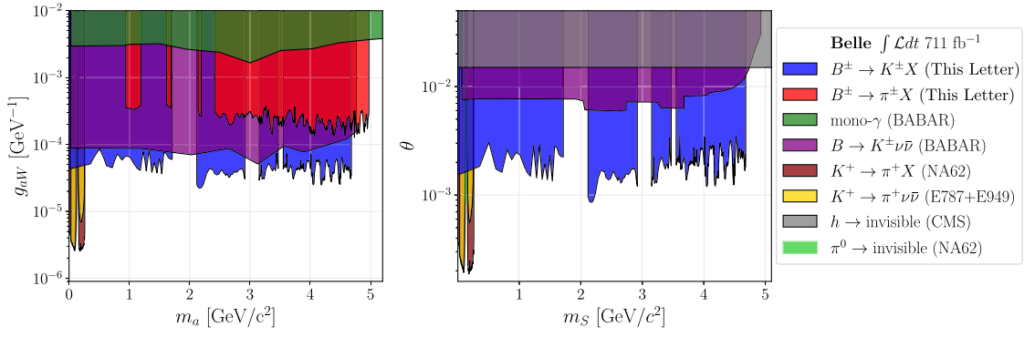
FIG. 3. Excluded regions for m_{X_{\text{inv}}} up to 5.1 GeV/c 2 at 90% CL shown for: (a) the coupling g_{aW} in the invisible ALP scenario from Ref. [28], and (b) the mixing angle \theta for the dark scalar in the missing energy scenario from Ref. [43]. Exclusions from BABAR [50,91], NA62 [21,23], E949 [24], and CMS [92] are overlaid for comparison.
