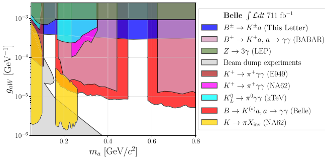
FIG. 4. Limits on the coupling strength g_{aW} assuming the ALP decays via a \rightarrow \gamma\gamma , including the constraints from other experiments presented in Ref. [28], with the addition of more recent constraints that appear in Ref. [14].
