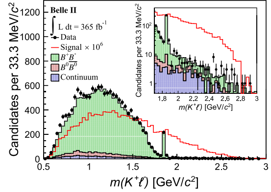
FIG. 1. Distribution, with simulation overlaid, of opposite-charge kaon-lepton mass in Belle II events. Logarithmic vertical scale in the inset assists visualization of the high kaon-lepton mass analysis region.
