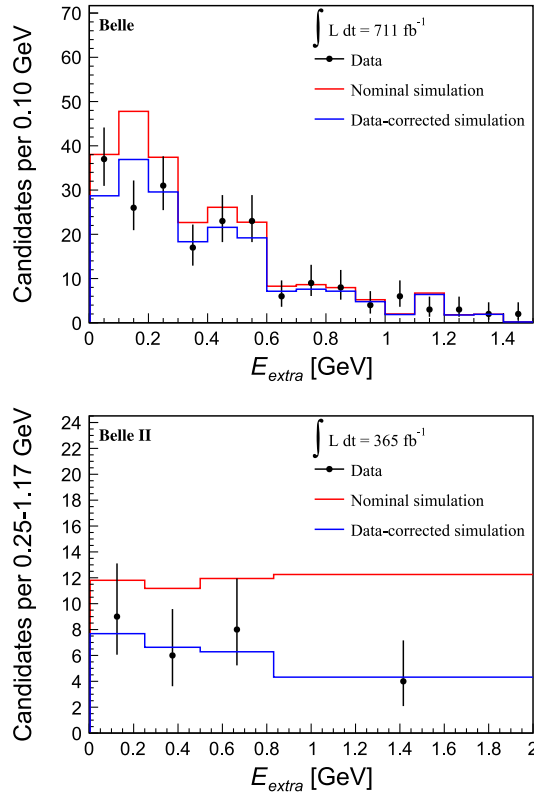
FIG. 2. Distributions of E_{\text{extra}} for (circles) data and (histograms) simulation (red) before and (blue) after the linear-scaling fit for (top) Belle and (bottom) Belle II events populating the partner- B M_{bc} sideband.
