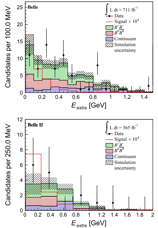
FIG. 3. Distributions of E_{\text{extra}} after final selections in (top) Belle and (bottom) Belle II data. Expectations based on corrected simulation for backgrounds and for 10^4 \times -enhanced SM signal [1] are overlaid.
