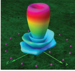
Intensity pattern of a radio beam generated by two circular arrays of vector antennas (purple dots). The pattern corresponds to the orbital angular momentum l = 1 found in Laguerre-Gauss laser beams. See article 087701.
