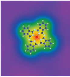
Topography of an MnPc molecule adsorbed on a Pb island. The Kondo resonance can be tuned by manipulating the electronic structure of the host Pb island. See article 256601.
