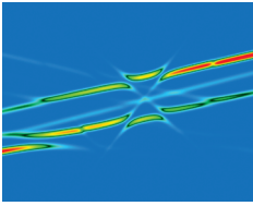
Calculated photoluminescence intensity (from blue to red) of the neutral exciton from a Mn-doped InAs quantum dot, with magnetic field (horizontal, \pm 3 T) plotted against detection energy (vertical, \pm 0.75 meV). The exchange couplings among Mn, electron, and hole spins cause the multiple anticrossings. See article 247209.
