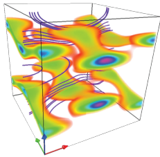
A dynamo mode with a wavy spatial distribution of magnetic energy and field lines, from full magnetohydrodynamic simulations of subcritical dynamo bifurcation. See article 224501.
