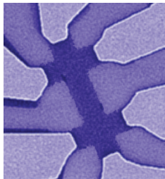
Scanning electron microscopy image of a graphene multiterminal device used to measure quantum Hall activation gaps. See article 206803.
