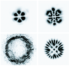
Light intensity distributions for spatiotemporal pulses generated in a ring cavity with a liquid crystal gain medium. See article 023901.
