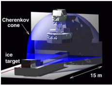
ANITA balloon payload set up to detect radio Cherenkov emission from particle showers produced when a high energy electron beam strikes a seven ton ice target. See article 171101.
