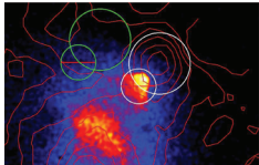
x-ray image of the Bullet Cluster and dark matter gravitational potential (red curves). Emissions from the densest region (white circles) are compared with a reference region (green circles) to bound the lifetime of axionic dark matter. See article 131301.
