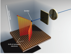
Experimental setup to detect ground state two-proton decay from long-lived ^{45}\text{Fe} in a time-projection chamber. See article 102501.
