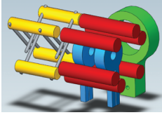
Schematic of a magnetoelectrostatic trap used to confine 3000 neutral ground state OH molecules at 30 mK. See article 253002.
