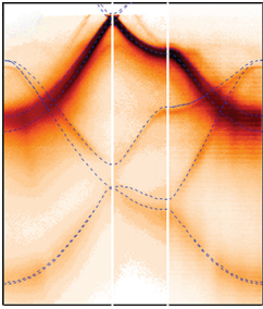
Band structure of bilayer graphene imaged through photoemission intensity mapping. White lines indicate directions of high symmetry and blue dashed lines are obtained from theory. The study finds a transition from 2D to bulk behavior in multilayer graphene. See article 206802.
