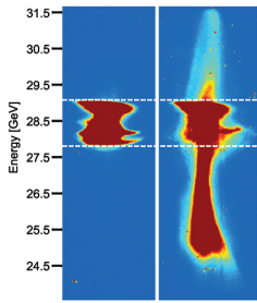
Energy spectrum of a relativistic electron beam before and after propagation through a plasma, showing the multi-GeV wakefield acceleration of particles. See article 054802.
