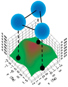
Model plot of the density distribution (red-green areas) of an excess neutron in a ^{14}\text{C} nucleus. A molecular-orbital calculation suggests that this nucleus consists of three alpha clusters (blue spheres) forming an equilateral triangle in the xy plane, surrounded by two additional neutrons. See article 142501.
