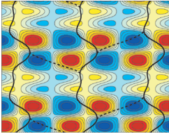
Angle-time plot of a model potential for the direction of a magnetic dipole (a nanoparticle in a ferrofluid) placed in an oscillating magnetic field. Full lines are long-time, deterministic solutions; dashed lines show noise-induced transitions between these. An average rotation of the particle results from different probabilities for forward- and backward-slip transitions. See article 060602.
