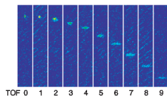
False-color absorption images of ultracold ytterbium atoms after release from an optical trap; the time-of-flight axis is in milliseconds. The atoms expand anisotropically, a signal that they have formed a Bose-Einstein condensate. This is the first observation of the Bose-Einstein condensation of atoms in spin-singlet states. See article 040404.
