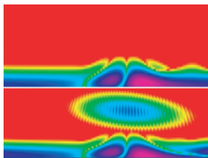
Color plots of the spectral intensity of radiation emitted in a simulated electron-ion collision for full (top) and for partial (bottom) ionization; time is along the horizontal axis. The bottom plot shows an attosecond radiation pulse due to "stimulated recombination", the result of a freed electron reencountering the ion and interfering with itself in the ground state. See article 173002.
