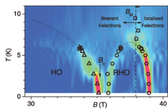
Phase diagram and magnetic-susceptibility plot of the strongly correlated metal \text{URu}_2\text{Si}_2 , showing the "hidden order" (HO) and field-induced reentrant (RHO) phases. "Hidden order" refers to a yet-unidentified order parameter, while the RHO phase is thought to be created at a magnetic-field-tuned quantum critical point. See article 096402.
