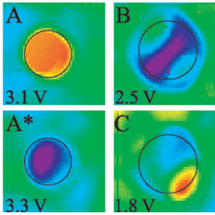
STM conductivity images of single Pd atoms deposited on an \text{Al}_2\text{O}_3 surface, taken at the indicated voltages. Such images can probe how the electronic structures of isolated metal atoms are modified by defects in the oxide surface. The apparent sizes of the atoms are indicated by the circles. See article 046808.
