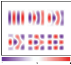
Simulation of a TE state magnetic field in a polaritonic photonic crystal for six closely-spaced frequencies. The nodal structure of the field mutates from one pattern to another. See article 196402.
