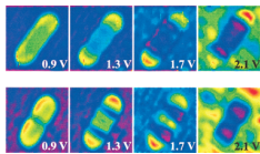
STM conductance images of quantum well states along an 11-atom Au chain on a NiAl substrate (top). The bottom images show how these states are disturbed when the chain absorbs a CO molecule, which disrupts the delocalization of electron-density waves in the chain. See article 186102.
