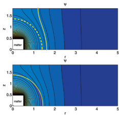
Contour plots for the metric of a hypersurface in a 5D "black-object" spacetime, compactified in the vertical direction. As the scale of the compactified dimension is varied, the horizon topology shows an abrupt phase transition, changing from cylindrical (top, corresponding to a nonuniform black string) to spherical (bottom, corresponding to a black hole). See article 171301.
