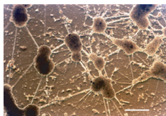
Microphotograph of in vitro neuron cells after 7 days of growth and self-organization. At low cell densities (not shown), the cells are distributed uniformly over the substrate; at the higher cell density depicted, the cells spontaneously migrate to form a network of clusters connected by bundles of axons. (White scale bar = 500 microns.) See article 168101.
