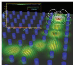
Illustration of a proposed micron-scale waveguide, showing nearly perfect, diffractionless transmission of an EM signal through a right angle. The electric field intensity, vectors, and equal-intensity contours are shown in light colors; the inset shows the calculated transmission and reflection properties of the bend. See article 123901.
