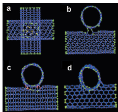
Numerical simulation of the merging of two carbon nanotubes. The starting configuration is shown in a top view in (a). Side views of the merging process are shown in (b) at 10 ps, (c) at 100 ps, and (d) at 220 ps. See article 075505.
