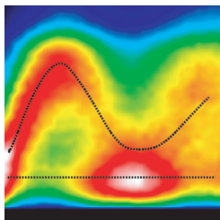
Contour plot of x-ray scattering intensity for water in a hydrated protein crystal from a molecular-dynamics simulation. The figure shows two Brillouin sound modes (dotted lines) in the interfacial water, corresponding to ordinary and fast sound in liquid water. See article 275501.
