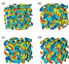
Lattice Monte Carlo simulation of the growth of a gyroid cubic phase in a triblock copolymer melt; the three different polymers making up the melt are indicated by the blue, red, and yellow areas, respectively. See article 205502.
