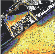
Map of the electrostatic potential caused by boron and phosphorous doping in a 0.35-micron silicon transistor, as determined by electron holography. The spatial resolution is 6 nanometers and the field of view is about 700 nanometers. See article 025502.
