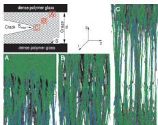
Simulation of crack propagation in an amorphous glassy polymer. The figures show, respectively, craze formation (A), deformation (B), and failure in front of the crack tip (C). See article 148304.
