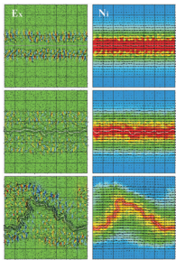
Simulated electric field (left) and ion density (right) showing the development in time (downward) of a current sheet instability. See article 095001.
