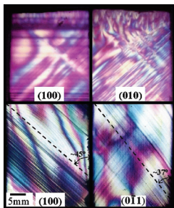
Front and back polarized light images of two strained \text{SrTiO}_3 crystals indicating shear bands on which intense plastic deformation occurred. See article 085505.
