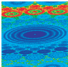
Quantum Husimi function for the sawtooth map in action angle variables. See article 227901.
