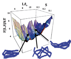
Simulated free energy of a 200-monomer chain as a function of crystal thickness ( L ) and orientational order parameter ( S ), dictating spontaneous selection of polymer crystal thickness. Ordered (valley) and disordered (saddle) configurations are shown. See article 218302.
