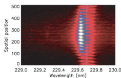
Light emission from doubly ionized carbon atoms in a Z-pinch plasma using an ICCD spectrometer. The Doppler shift from the C-III line at 229.7 nm (white line) shows the plasma's large axial velocity ( \sim 10^5 m/s) in the Z-pinch core, as well as a shear towards its edge. See article 205005.
