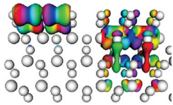
Kohn-Sham wave functions for two metallic edge states associated with Mo atoms at the edge of a MoS 2 nanostructure. See article 196803.
