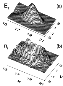
Numerical simulation plot of (a) the electric field and (b) the ion density inside a 'postsoliton' formed from the interaction of a high-intensity, ultrashort laser pulse with a plasma. See article 185004.
