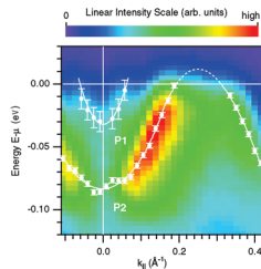
Experimental band structure map of bismuth measured by photoemission spectroscopy. See article 177602.
