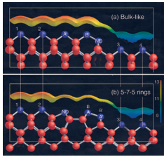
Side view of the atomic structures and theoretical STM images for D_B As/Ge steps. The blue balls are the As atoms and the red are the Ge atoms. See article 166104.
