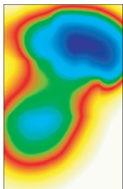
Calculated total energy of a Zn-rich CuZn random alloy indicating separate minima for the two hexagonal phases. (Average atomic radius versus c/a ratio.) See article 156401.
