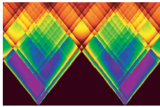
Spin-related fine structure in the differential conductance of a quantum dot as a function of gate (horizontal) and bias voltage. See article 146802.
