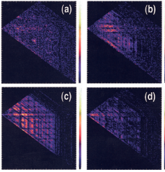
Change in coupling of high-frequency turbulence and low-frequency fluctuations through the low- to high-confinement transition. See article 135001.
