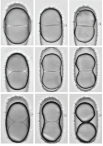
Droplet-encapsulated gels (DEGs) morphologies shown for different values of the liquid fraction (horizontal) and the elastocapillary number (vertical). [S. Saita et al. , Phys. Rev. Lett. 137 , 148203 (2026)]
