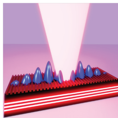
Supersolid emission pattern (blue) from a photonic crystal waveguide vertically pumped by a continuous wave source. Selected for an Editors' Suggestion. [Davide Nigro et al. , Phys. Rev. Lett. 134 , 056002 (2025)]
