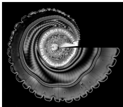
Time-lapse reconstruction of interference patterns from a spreading oil film during evaporation of an oil-in-water emulsion drop. [T. Dong et al. , Phys. Rev. Lett. 133 , 174001 (2024)]
