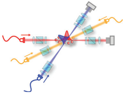
Experimental setup for simultaneous trapping of two optical pulses. [U.-S. Kim and Y.-H. Kim. Phys. Rev. Lett. 129 , 093601 (2022)]
