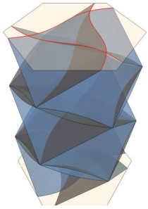
Energy bands of chiral zigzag modes in minimally twisted bilayer graphene. [C. De Beule, F. Dominguez, and P. Recher, Phys. Rev. Lett. 125 , 096402 (2020)].
