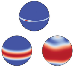
Heat maps of a neutron star crust within a neutron star binary system at three different stages of the inspiral phase. [Zhen Pan et al. , Phys. Rev. Lett. 125 , 201102 (2020)]
