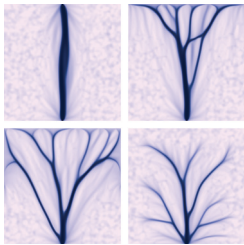
Simulated branching flow patterns of a fluid forced through a brittle, erodible medium with different boundary conditions. Selected for an Editors' Suggestion. [Nicholas J. Derr et al. , Phys. Rev. Lett. 125 , 158002 (2020)]
